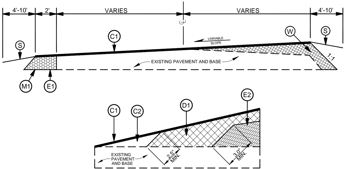
WEDGING DETAIL
